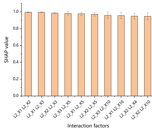
Figure 1. Interaction factor variables with the top ten largest SHAP values based on the GWRF model
