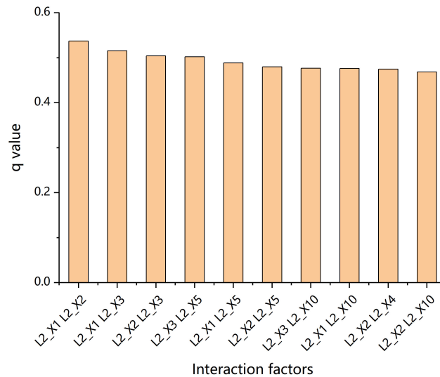
Figure 2. Interaction factor variables with the top ten largest q values based on the GD model
