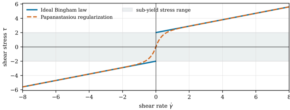
Figure 1. Ideal Bingham response and a smooth Papanastasiou approximation
