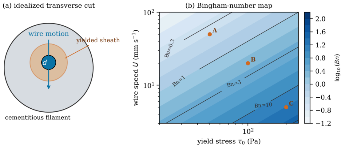
Figure 2. Proposed wire-cutting object and illustrative dimensionless operating map
