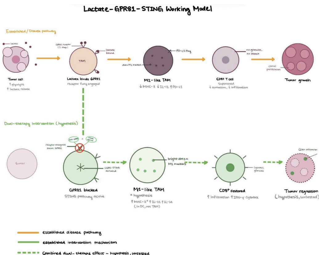
Figure 1. Working model of lactate-GPR81-STING signaling in tumor-associated macrophages and its consequences for CD8 + T cell-mediated tumor control
