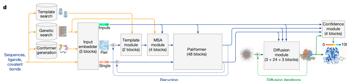
Figure 1. The overall architecture of AlphaFold3 [3]
