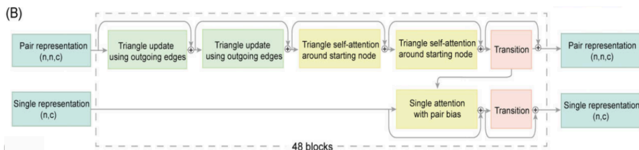
Figure 2. Working mechanism of the diffusion module in AlphaFold3 [3, 5]
