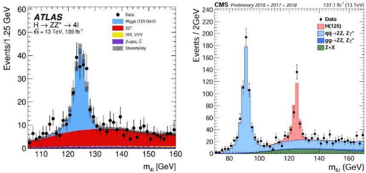
Figure 2. Mass distributions of Higgs boson candidate events in the ATLAS and CMS experiments [4, 5]
