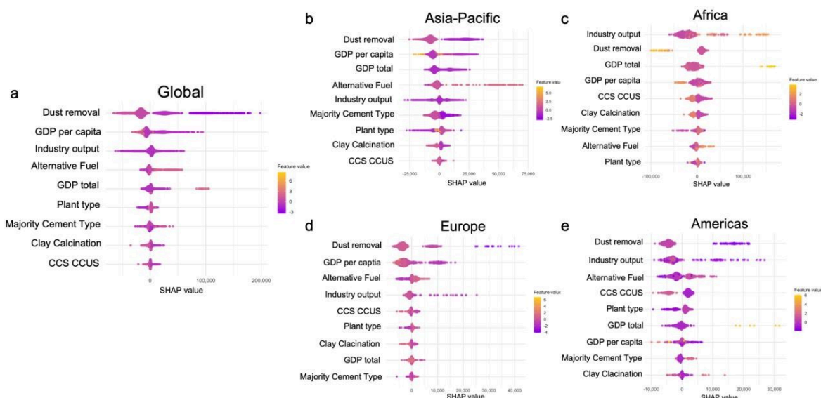
Figure 4. SHAP-based attribution of cement-related REE emission drivers. a, Global SHAP results for the random forest model. b–e, Regional SHAP results for Asia-Pacific, Africa, Europe and the Americas. Dust removal, industrial output, GDP-related variables and low-carbon technology indicators explain most spatial variation in predicted REE emissions. SHAP, Shapley additive explanations
