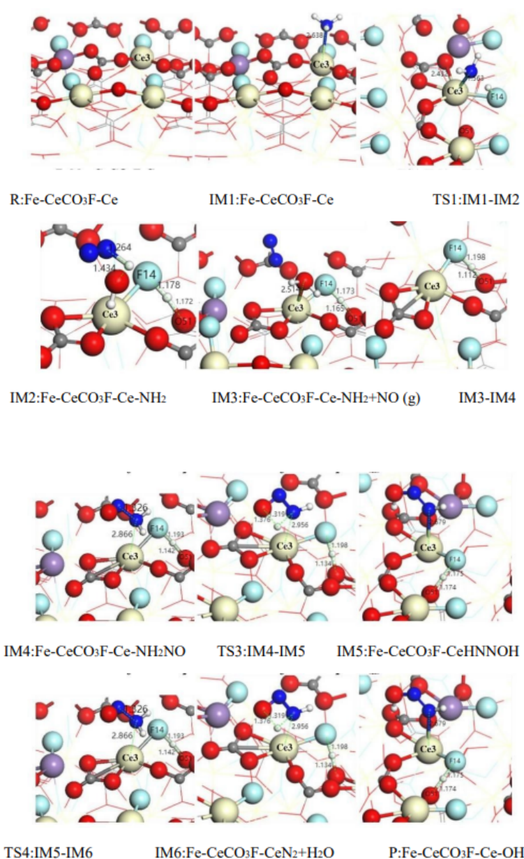
Figure 5: Structural diagrams of intermediates along the reaction pathway following the Eley-Rideal (E-R) mechanism at the \text{Fe-CeCO}_3\text{F-Ce} site
