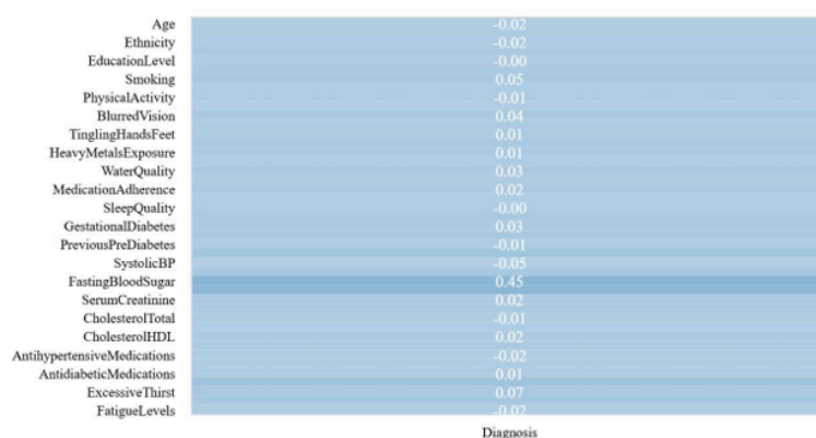
Figure 1: Visualization graph of Spearman correlation (picture credit: original)
