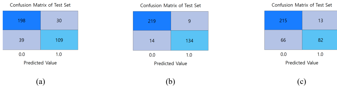
Figure 2: Confusion matrix diagram of models (picture credit: original)
