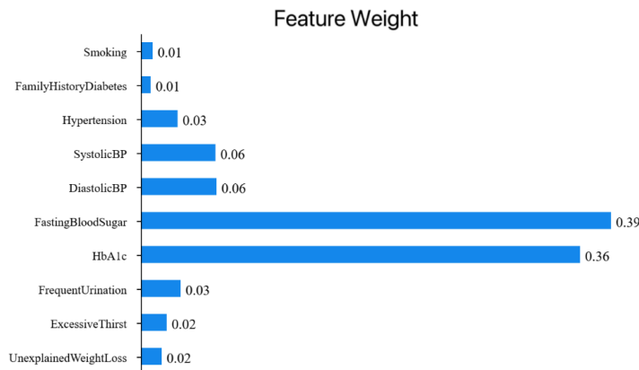
Figure 4: Feature weight of RFNN model (picture credit: original)
