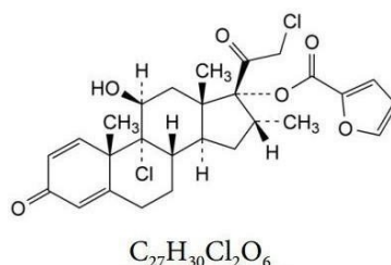
Figure 4: Structure and chemical formula of mometasone furoate
