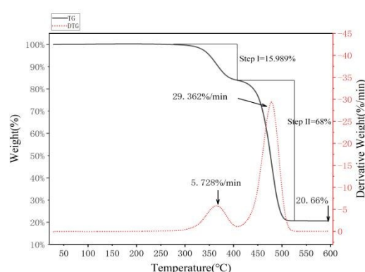
Figure 1: Thermogravimetric analysis curve of EVA film
