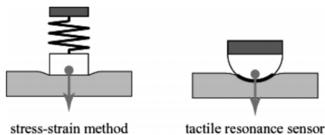
Figure 2: Comparison of the stiffness measurement methods
