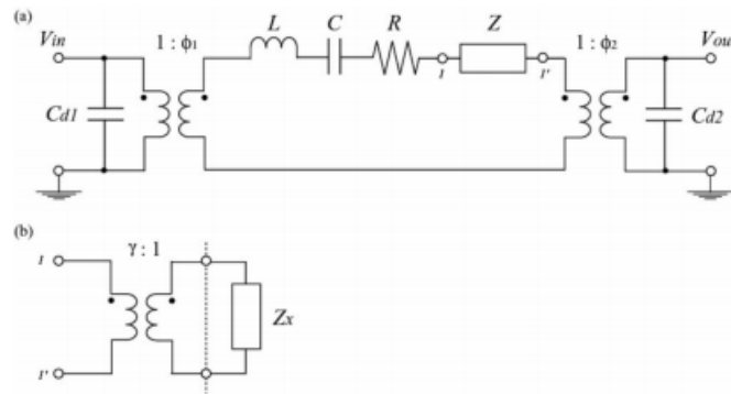
Figure 1: Equivalent circuit of the tactile resonance sensor [2]
