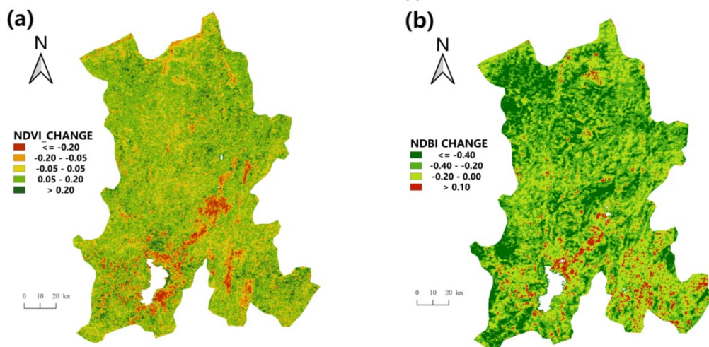
Figure 4: (a) NDVI change (2000-2022) (b)NDBI change (2000-2022)
