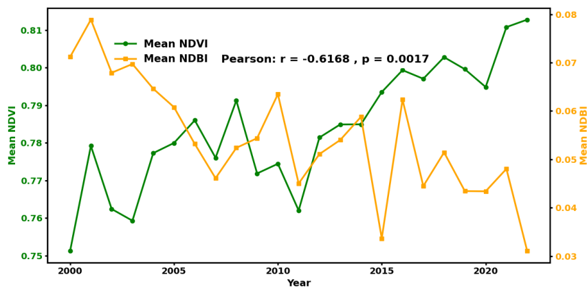
Figure 3: Correlation of NDVI&NDBI (2000-2022) in Kunming
