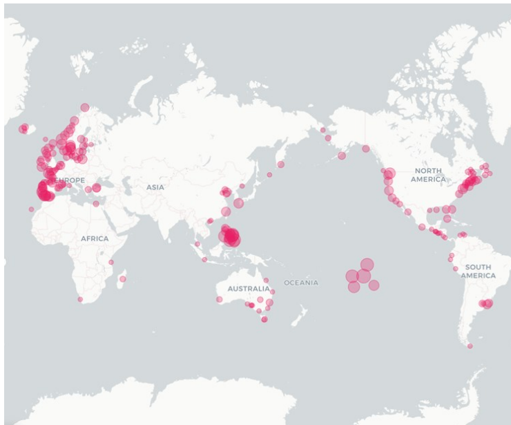
Figure 1: The global HAB events reports distribution since 2020 [5]
