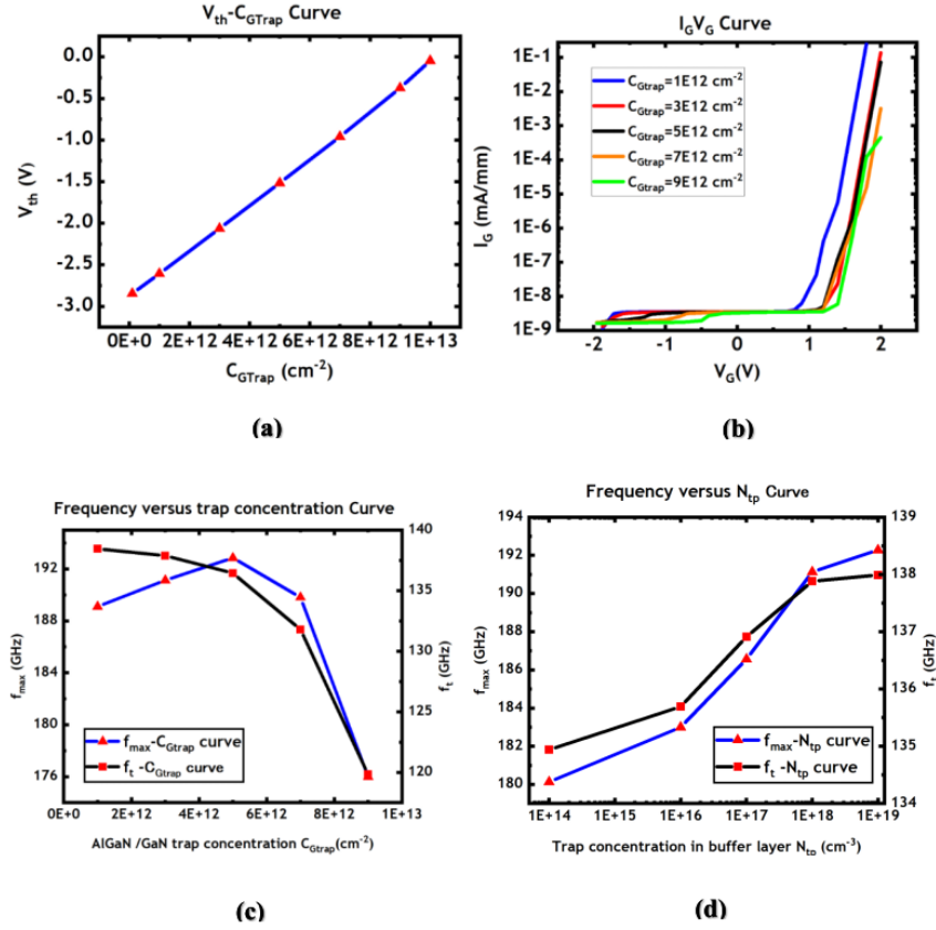
Figure 4: The (a) threshold voltage; (b) I_G - V_G curve; (c) cut-off frequency and maximum oscillation frequency as a function of interface traps concentration and (d) cut-off frequency and maximum oscillation frequency as a function of traps concentration in GaN buffer layer
