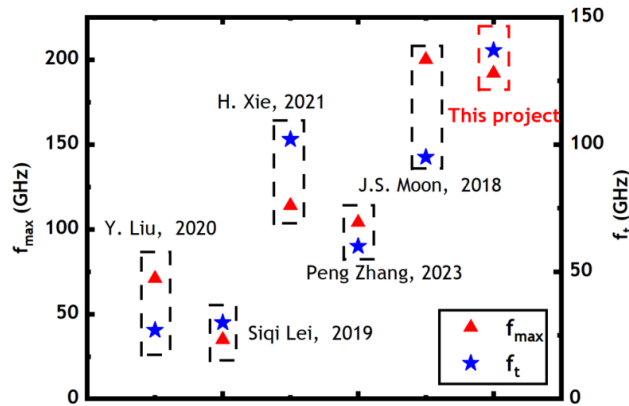
Figure 5: Comparison of GaN HEMTs frequency performance between our project and other paper
