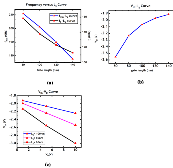
Figure 3: (a) maximum oscillation frequency and cut-off frequency; (b) threshold voltage; (c) drain-induced barrier lowering effect of device with different gate length
