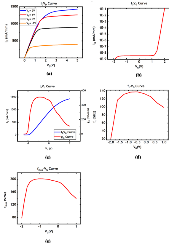
Figure 2: The (a) I_D - V_D curve; (b) I_G - V_G curve; (c) I_D - V_G curve; (d) f_t - V_G curve and (e) f_{max} - V_G curve of T-gate GaN HEMT
