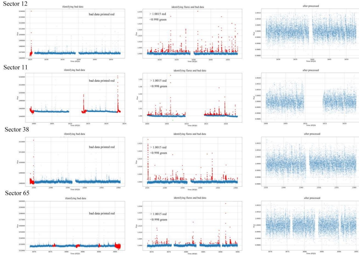
Figure 1: The first column indicate the interval of bad data deleted. The second column is the lightcurves with flares printed red and bad data printed green. The last column are the lightcurves processed and used for BLS in 2.2
