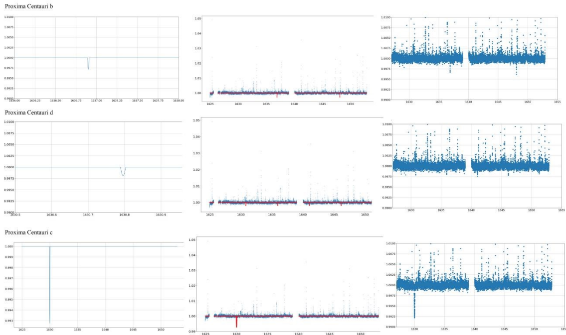
Figure 3: The first column shows single simulated transits for the three planets. The second column is the combined initial lightcurves with our simulated ones, with simulated signals printed red. The third column lays the combined lightcurves in scatter form
