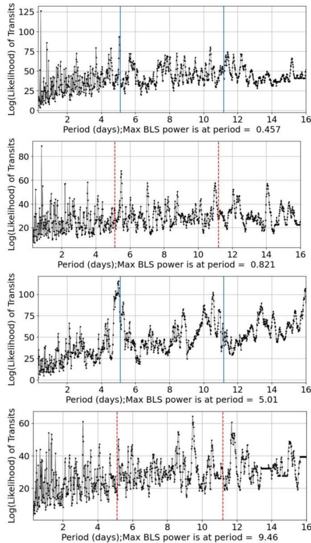
Figure 2: The BLS graph for sector 12,11,38,65 from the top to the bottom. Maximum BLS power period is labeled on the axes
