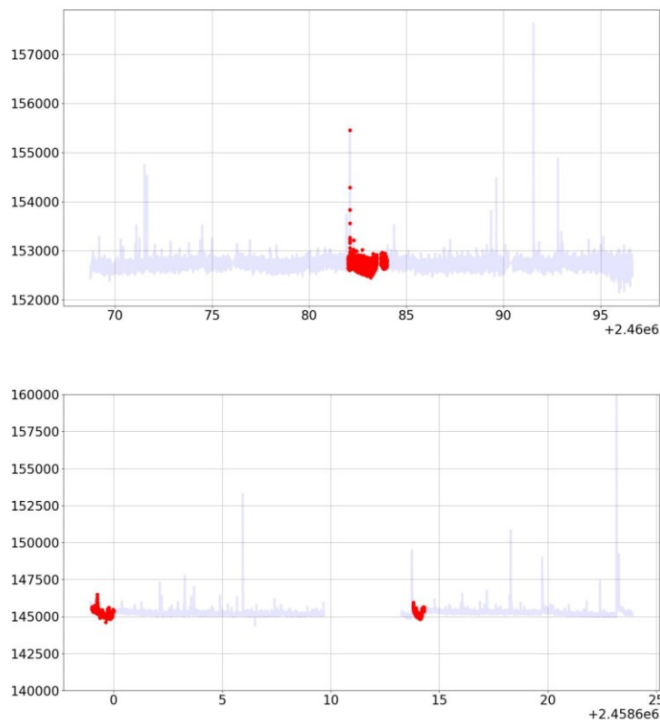
Figure 5: Some region where indicate a transit trend
