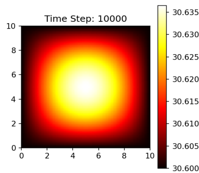
Figure 2: Temperature evolution at time step 10,000
