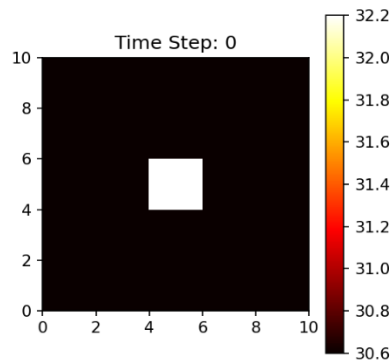
Figure 1: Initial temperature distribution at time step 0
