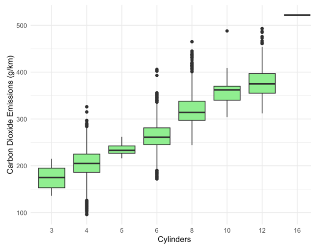
Figure 1: Distribution of CO 2 emissions by cylinder count
