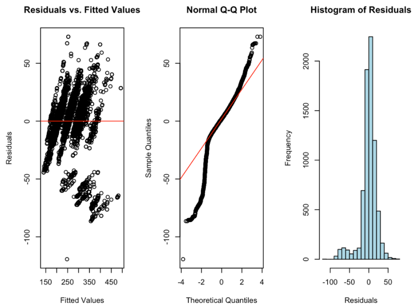
Figure 4: Residual analysis
