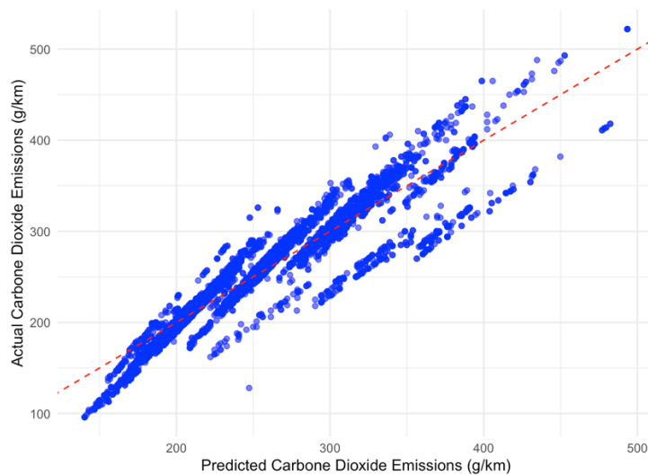
Figure 5: Predicted vs. actual CO 2 emissions
