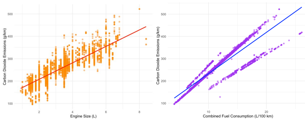
Figure 2: Engine size vs. CO 2 emissions and fuel consumption vs. CO 2 emissions
