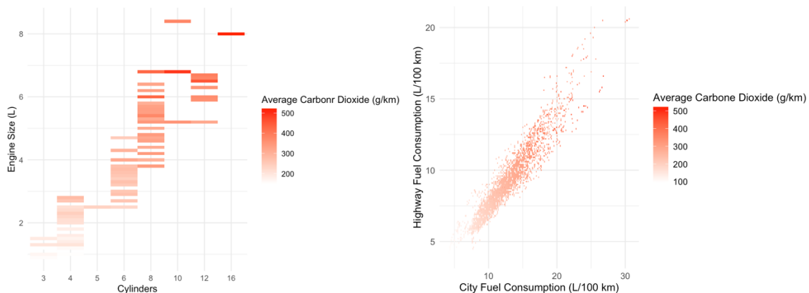
Figure 3: Heatmap of engine size vs. cylinders vs. CO 2 emissions and city vs. highway fuel consumption vs. CO 2 emissions
