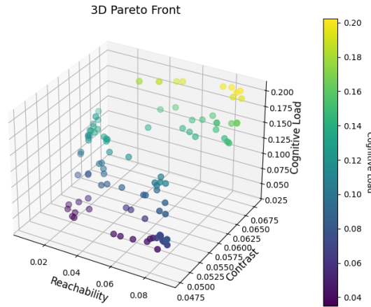
Figure 1: 3D Pareto front (wide-body aircraft)
