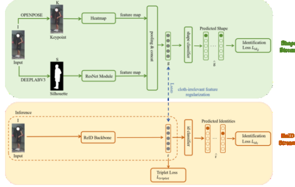
Figure 2. Structure of SKF-ReID involves the ReID Stream and Shape Stream, jointly trained with cloth-irrelevant feature regularization. The Shape Stream guides the ReID Stream to obtain clothing-agnostic representations, with the Shape Stream excluded during inference for efficiency.
