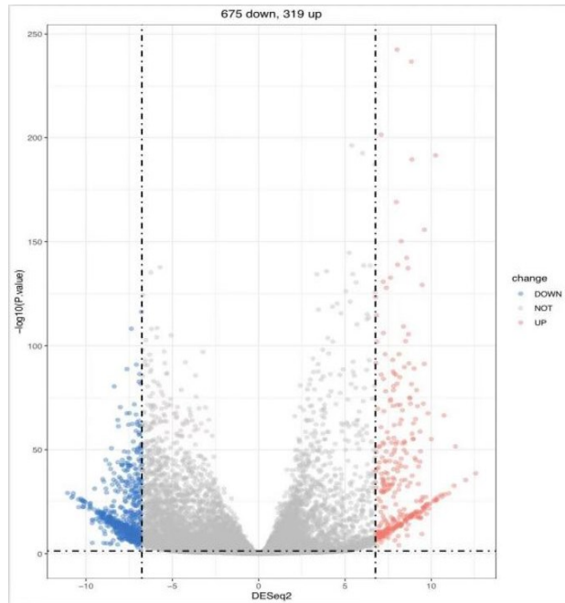
Figure 3. The volcano plot of differential expression genes in TBI.
