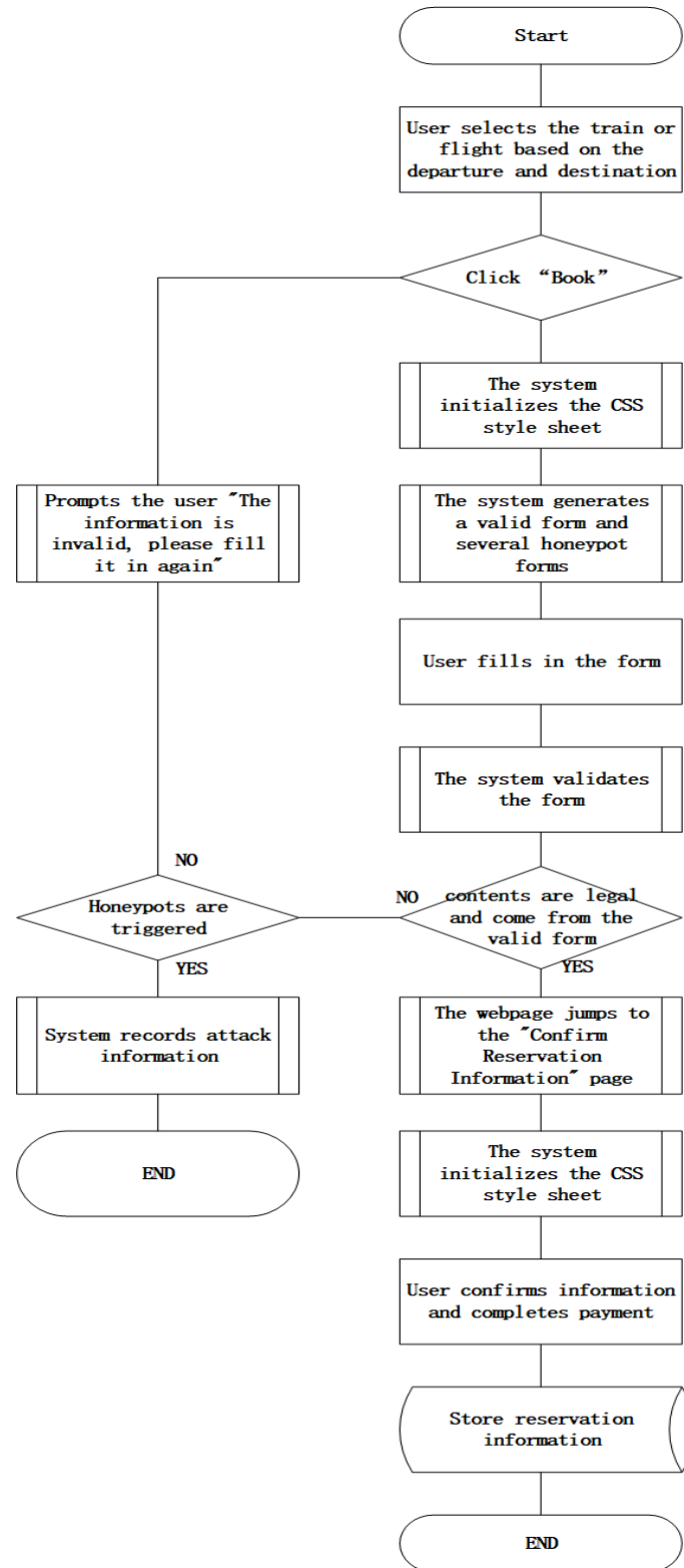
Figure 2. Model Architecture
