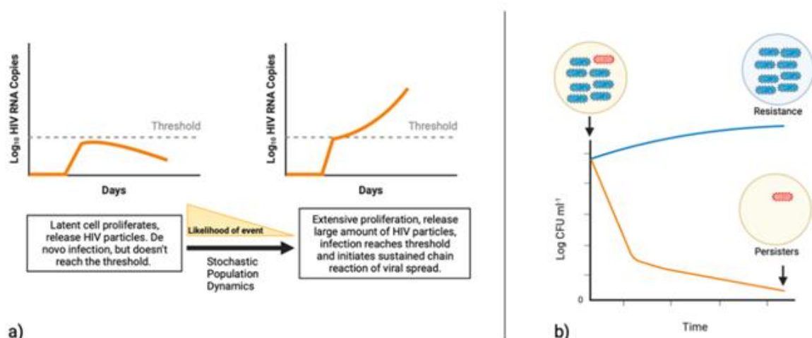
Figure 1. Stochastic model in HIV and bacteria. a) Stochastic transition to exponential HIV growth. The transition from latent to exponential growth state occurs when the initial virus release exceeds the critical growth threshold. The exponential growth state is rarer compared to the latent state; b) Growth pattern of antibiotics treatment of resistant bacteria and persisters. After the initial addition of antibiotics to a heterogeneous population of bacteria (yellow), the susceptible bacteria will be killed rapidly followed by a slower decrease in the colony forming units (CFU) as persisters (red) which occupy a small fraction of the population will survive (orange curve); With the addition of antibiotics to a homogeneous population of resistant bacteria (blue), there will be a continuous growth of bacteria population. Additionally, it is believed that SC population heterogeneity including variation in SC self-renewal and fate determination in an isogenic clone can be caused by both random intrinsic and extrinsic noise factors. This variability is crucial as it creates diversity in cellular functions as well as provides organisms with developmental plasticity and regenerative capabilities. Later sections will provide more detailed information on this topic.
